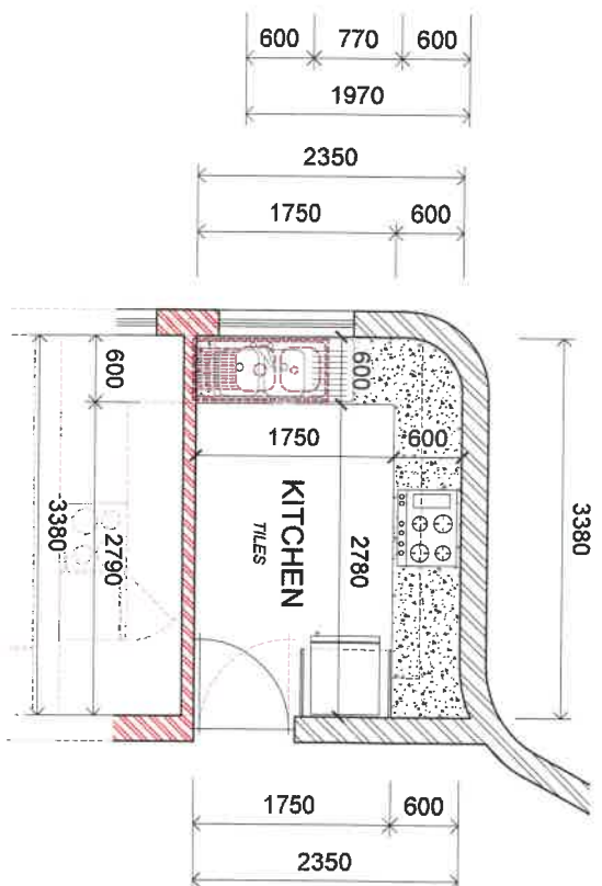
LAYOUT : UNIT 15 AND 16 SCALE 1:50
