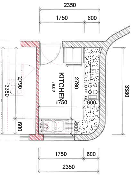
LAYOUT : UNIT 15 AND 16 SCALE 1:50
