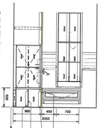
SECTION B SCALE 1:50
